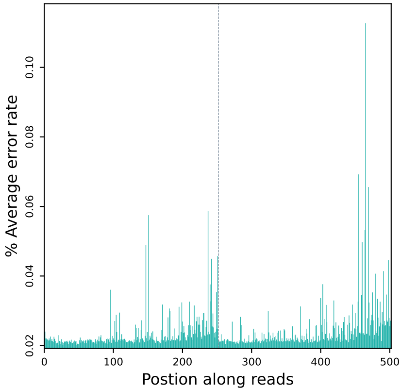
Error rate distribution along reads (R10802)
